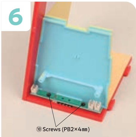
Tighten the ⑩ Screws (PB2×4mm) into the two holes in the Circuit Board to secure it in place.
