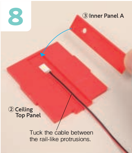
To prevent the cable from sagging, tuck it between the rail-like protrusions of the Ceiling Top Panel and fit ③ Inner Panel A from above.
