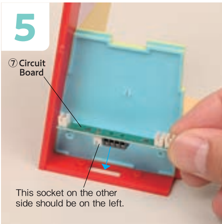
Assemble the ⑦ Circuit Board to the rear side of the Floorboard as shown.
